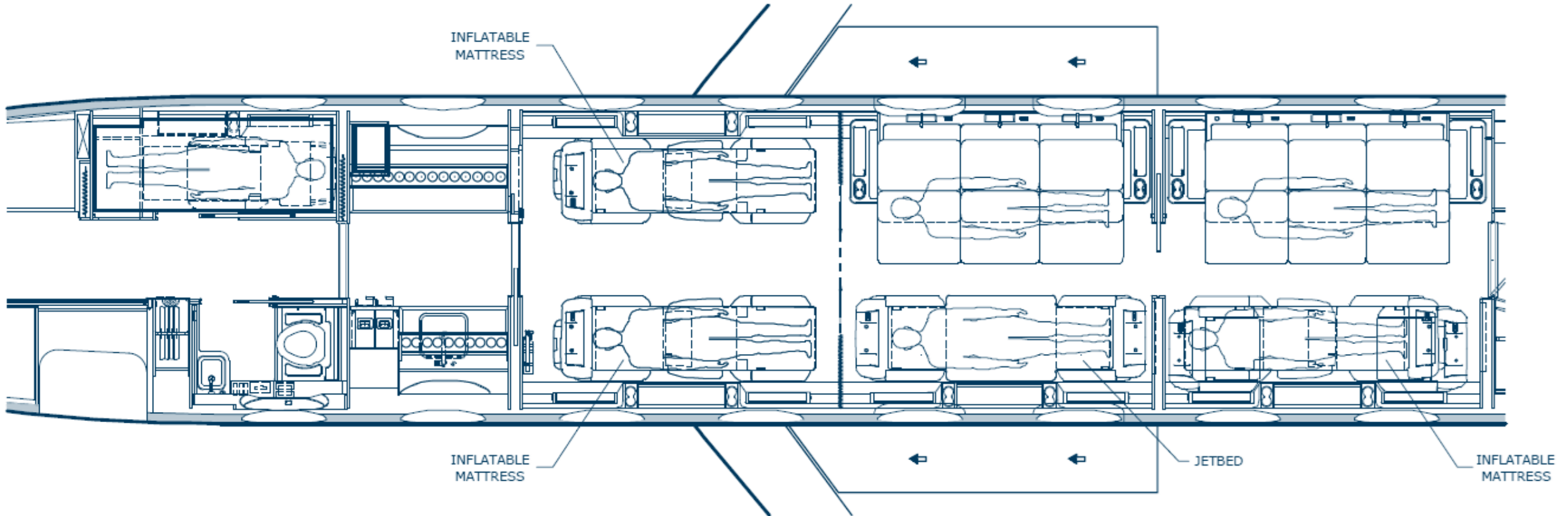
Berthing Plan View
